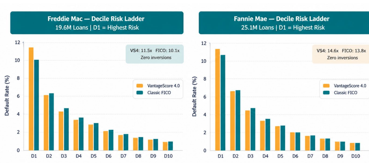
Figure 1.1: Decile Risk Ladders — VantageScore 4.0 vs. FICO Classic Score (Freddie Mac & Fannie Mae). Both models produce perfectly monotonic risk ladders with no inversions. VantageScore 4.0’s decile spread is marginally wider at both GSEs; quintile spreads converge. Source: Tables B.1, B.2 (Appendix B).
