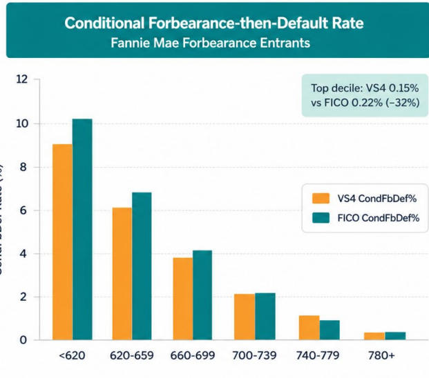
Figure 3.1: Decile spread expands during stress period across models (VantageScore 4.0: 19.6x; FICO Classic Score: 13.9x). VantageScore 4.0 Top Decile CondFbDef is 32% lower than FICO Classic Score at Fannie Mae. Source: Tables 1.5, 1.6, 2.5 (Source: Appendix D)
