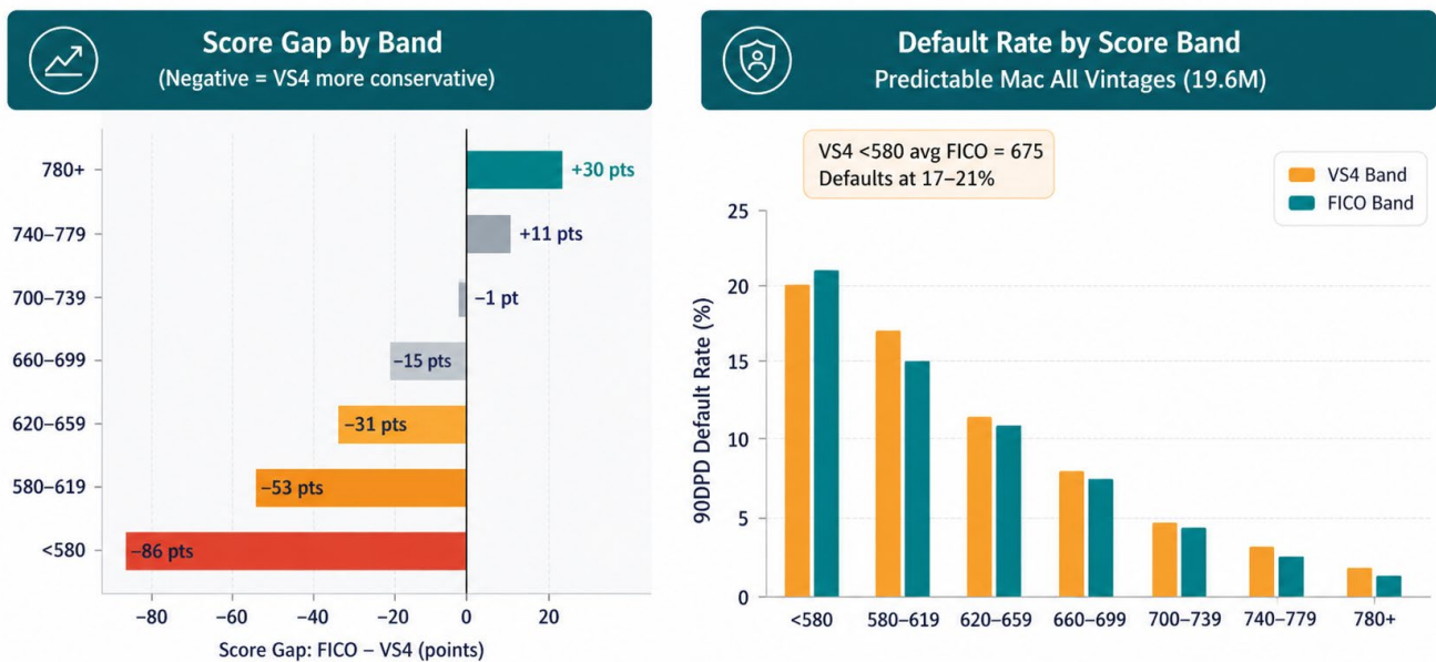
Figure 2.1: Lower Score Assignment in High-Risk Segments and Associated Default Rates
